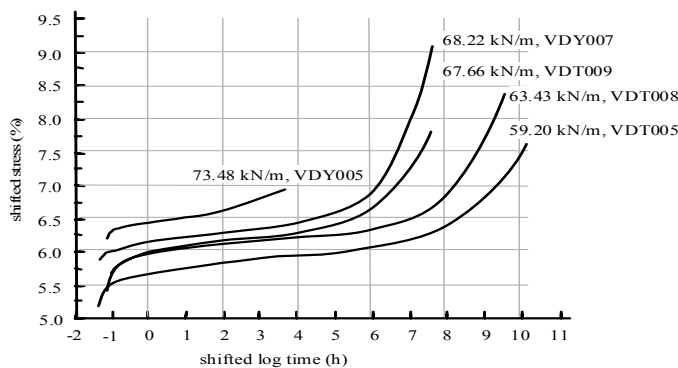
Figure 12, creep at high loads using SIM testing method.
