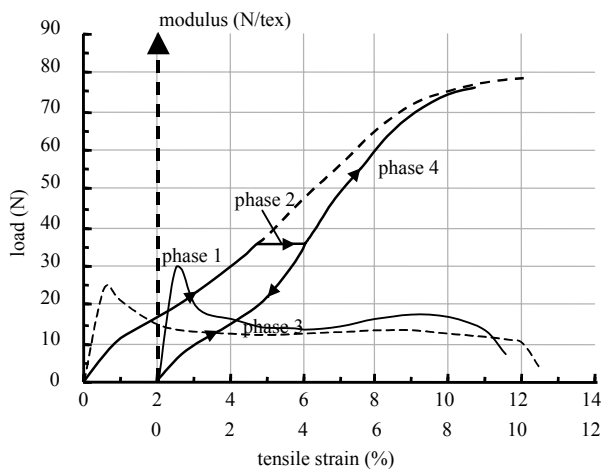
Figure 2. Loading path during creep tests, with phase 2 as continuous loading path (Voskamp 2001). Phase 1 and 2 cover the initial loading and creep phase. Phase 3 and 4 are the unloading and loading phase up to break. These last phases equal a stress strain curve with an origin at 2%.
