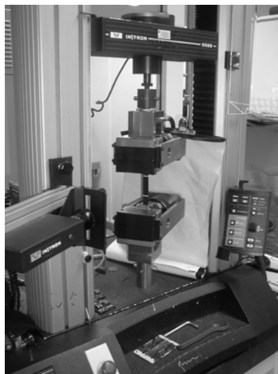
Figure 7, creep measurements with tensile loading device
