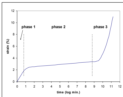
Figure 1 typical creep curve
