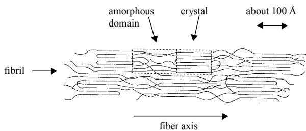
Figure 4. Physical structure of PET yarn (V.d. Heuvel, C.J.M.).
