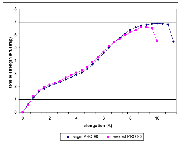
Figure 10, typical stress-strain figure
