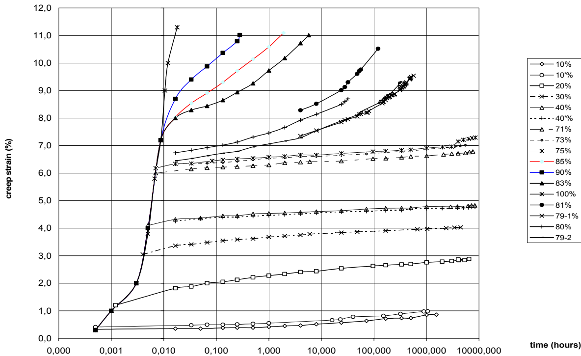
Figure 9 creep strain vs. time
