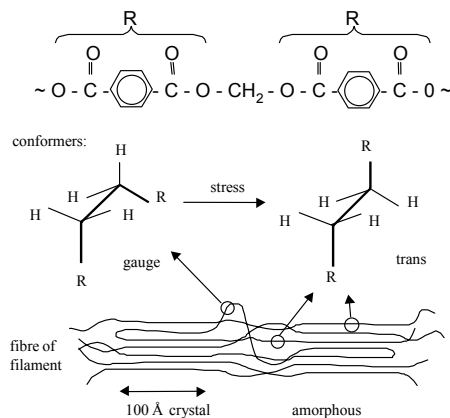
Figure 5. Molecular and physical structure of PET (V.d. Heuvel, C.J.M., 1993).
