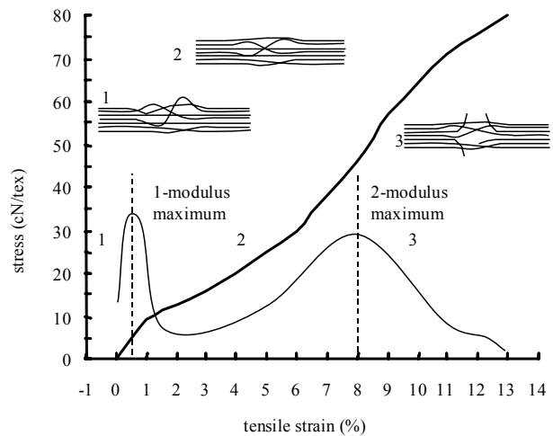
Figure 6. Molecular processes in the 3 regions (Voskamp W, 2001).
