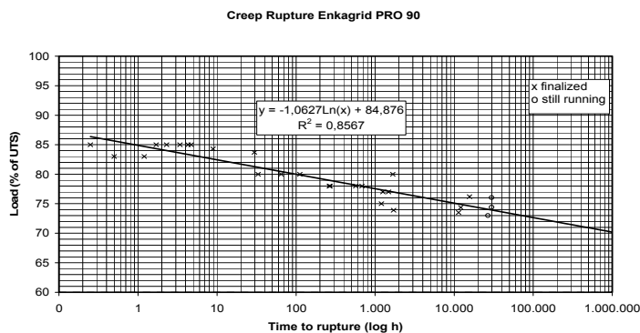
Figure 11 creep-rupture of 2 strips Enkagrid PRO90
