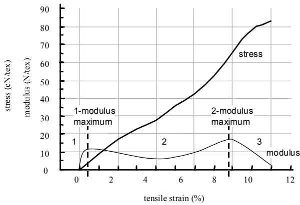
Figure 3. Typical stress-strain curve with modulus values (v.d. Heuvel C.J.M., 1993).
