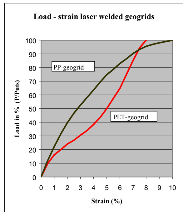
Figure 6. Normalized load-strain curves
