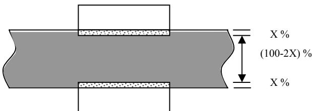
Figure 5. Sacrifice layer due to laser welding process
