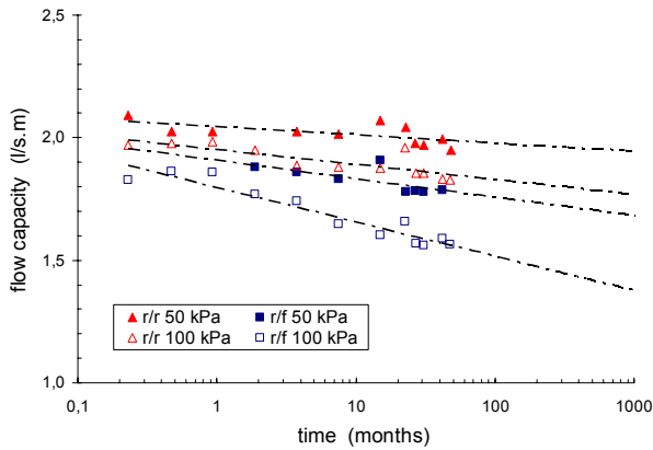
Figure 5. Influence of support on flow capacity of a TVT-GCO at 50 kPa and 100 kPa loading
