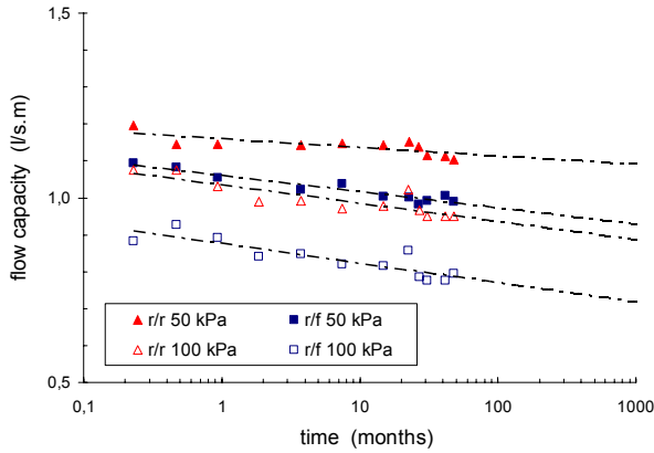
Figure 4. Influence of support on flow capacity of a MVM-GCO at 50 kPa and 100 kPa loading
