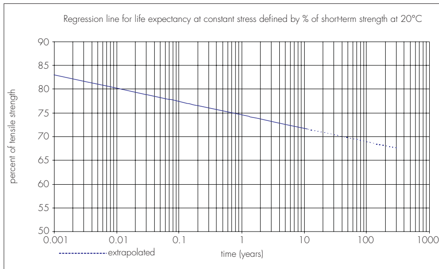
Figure 4 Time to rupture
